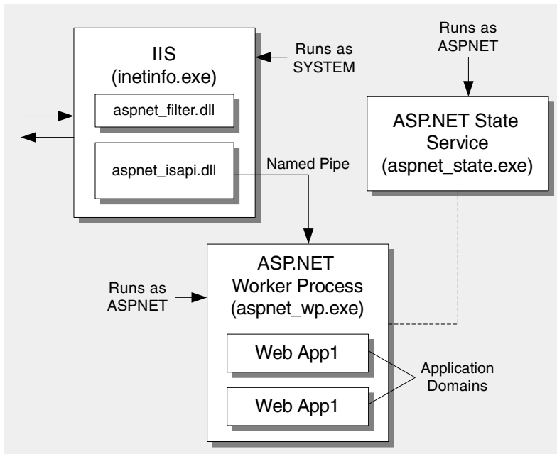
Figure 20.1 ASP.NET architecture on Windows 2000 with IIS 5
