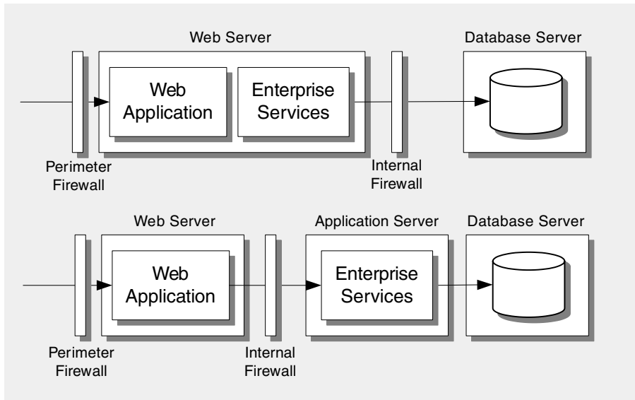
Figure 11.3 Enterprise Services typical deployment configurations
